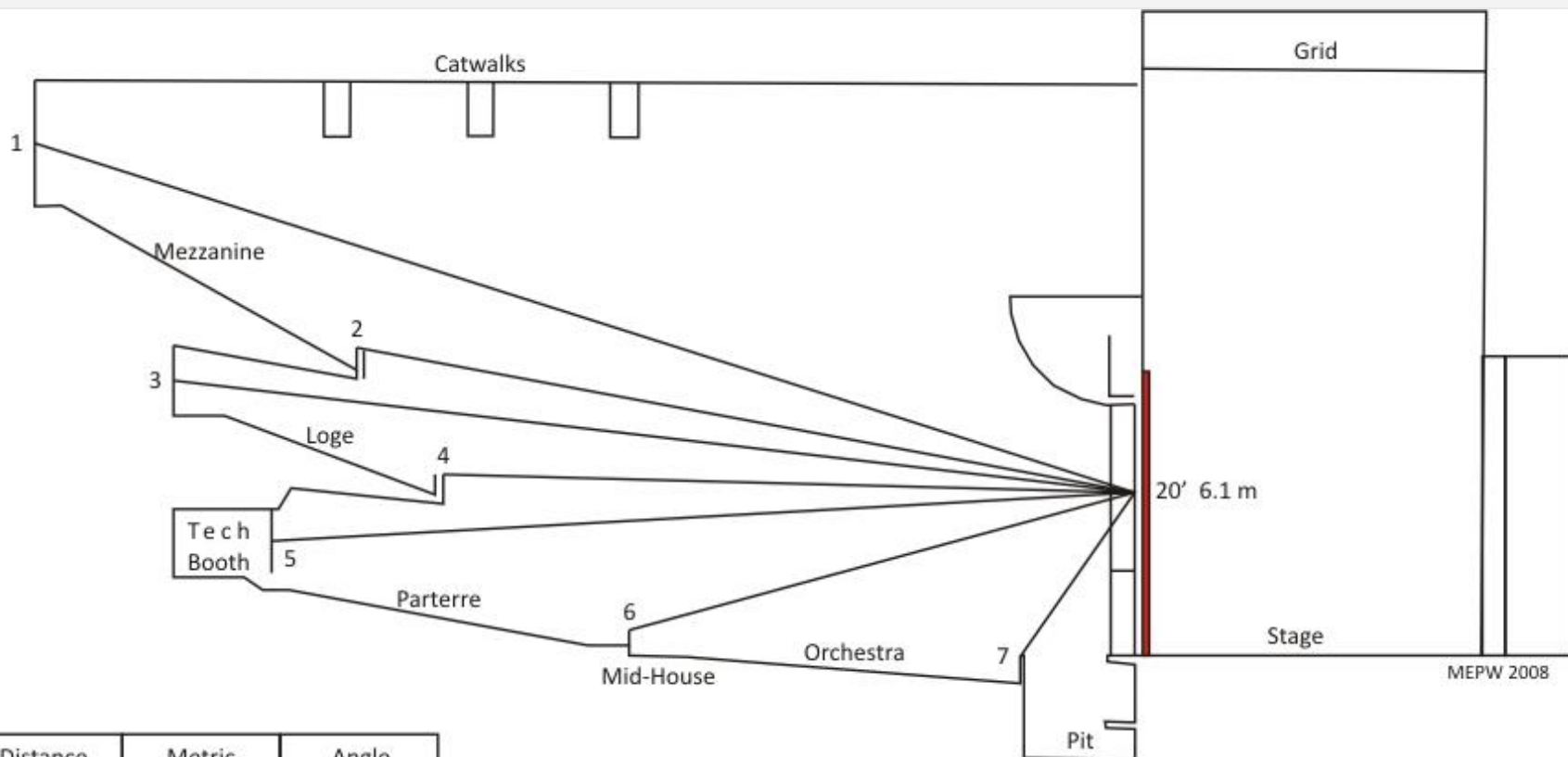
Classic Center Theatre Cross-Section with Distances and Inclination/Declination From Downstage Center at 20' above Deck
