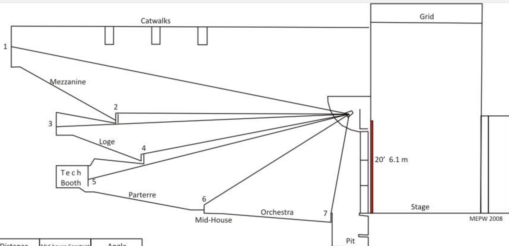
Classic Center Theatre Cross-Section with Distances and Inclination/Declination From Center Cluster Array
